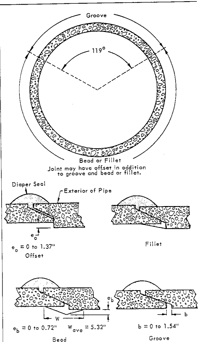
FIGURE 1: Cross-Section of Concrete Pipe Test Joints
